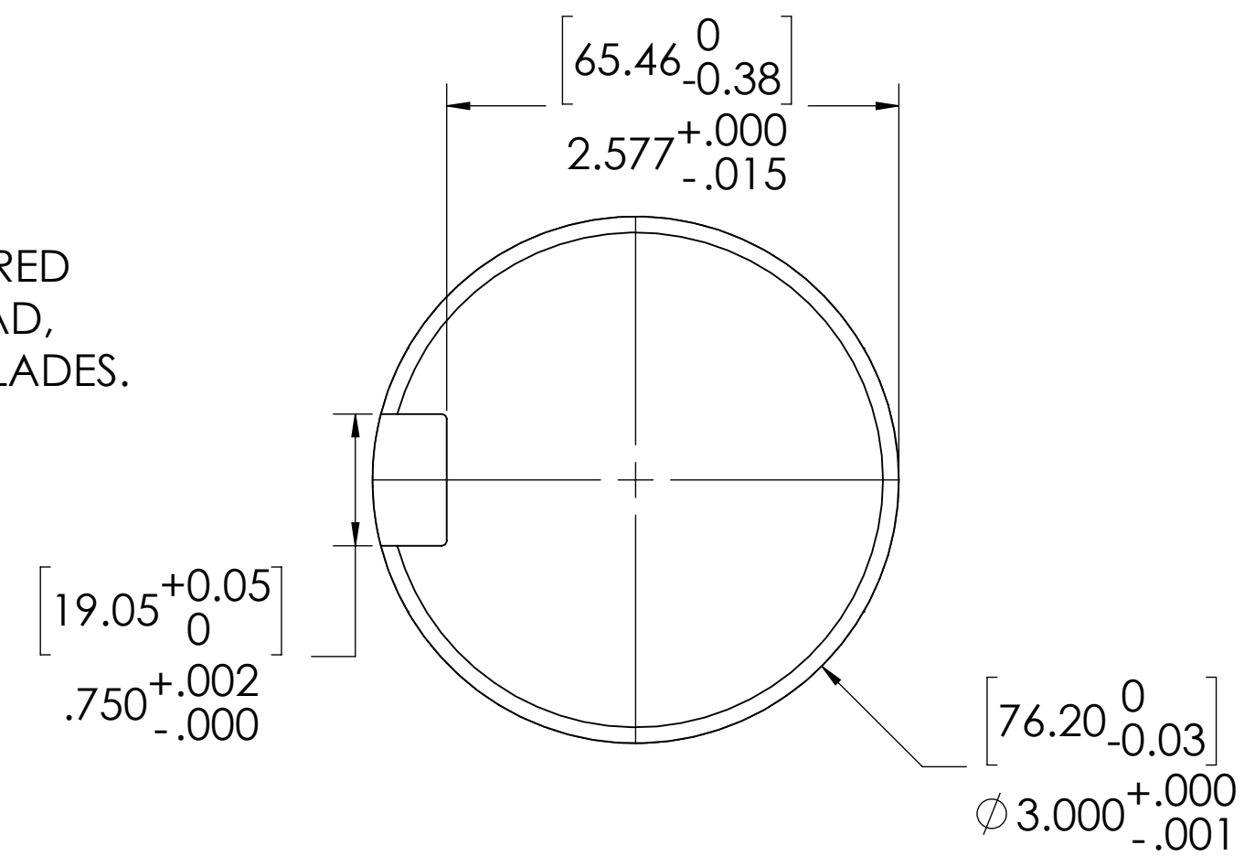
DETAIL OF ROTOR KEYWAY (BOTH ENDS)
